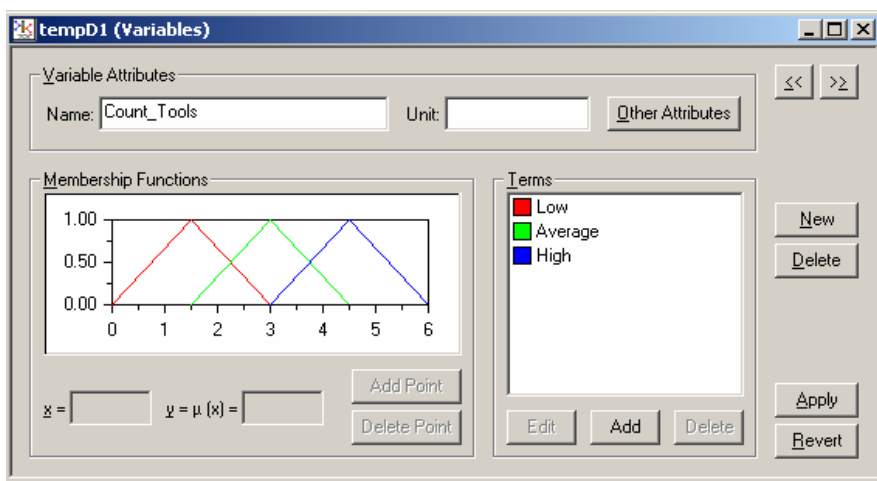
Data engine
